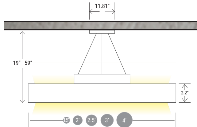
SUSPENDED/PENDANT
