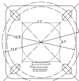
Anchor template
