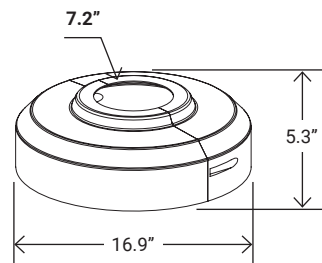
Base cover
