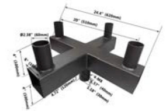
Quad 90° Horizontal Tenon Adapter NO. QT90-4T-D
