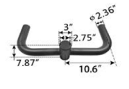
Double 180° Horizontal Tenon Adapter NO. RB2.5TR180H-D
