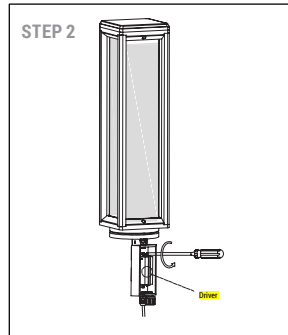
Unscrew the fixed metal strip and replace with new driver following the same wiring
