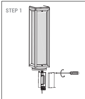
Unscrew the four screws of fixture
