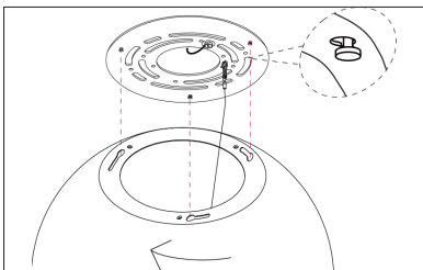
Install the lamp body.
