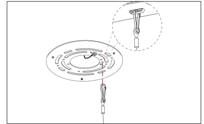
Connect the safety rope.
